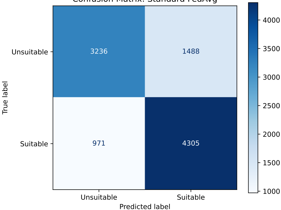
Confusion Matrix: Standard FedAvg
