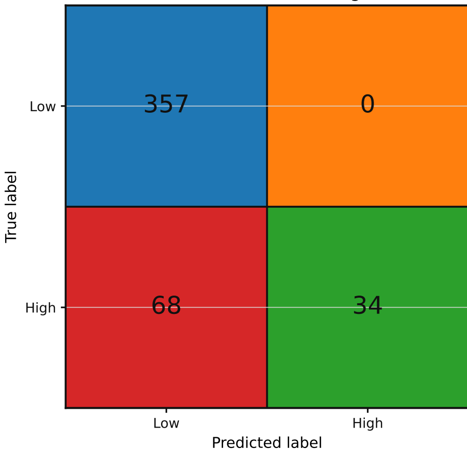
WESAD Confusion Matrix - AgHealth+
