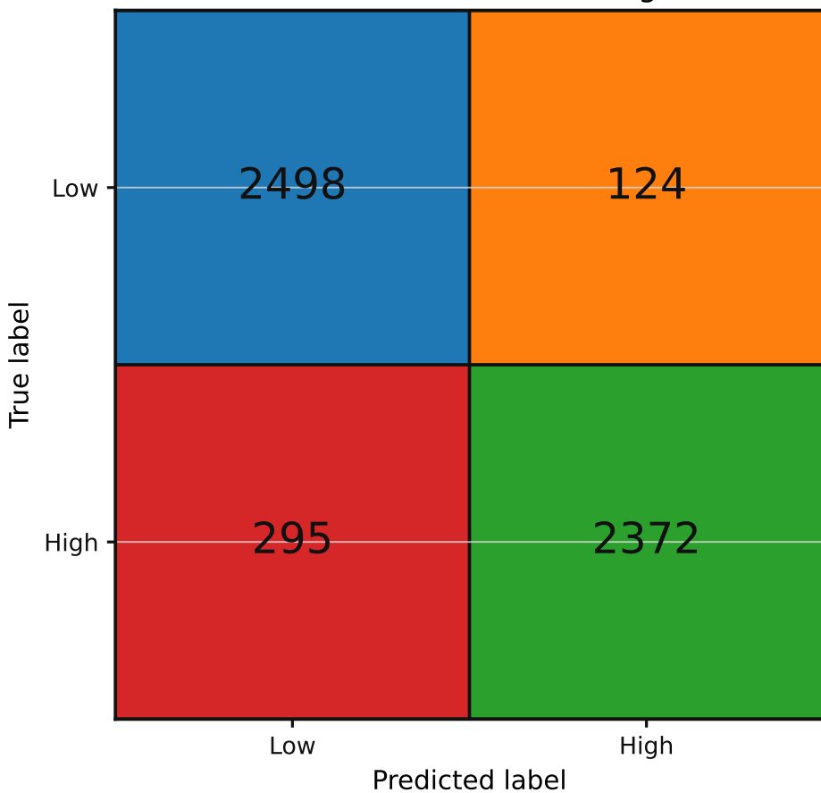
OhioT1DM Confusion Matrix - AgHealth+
