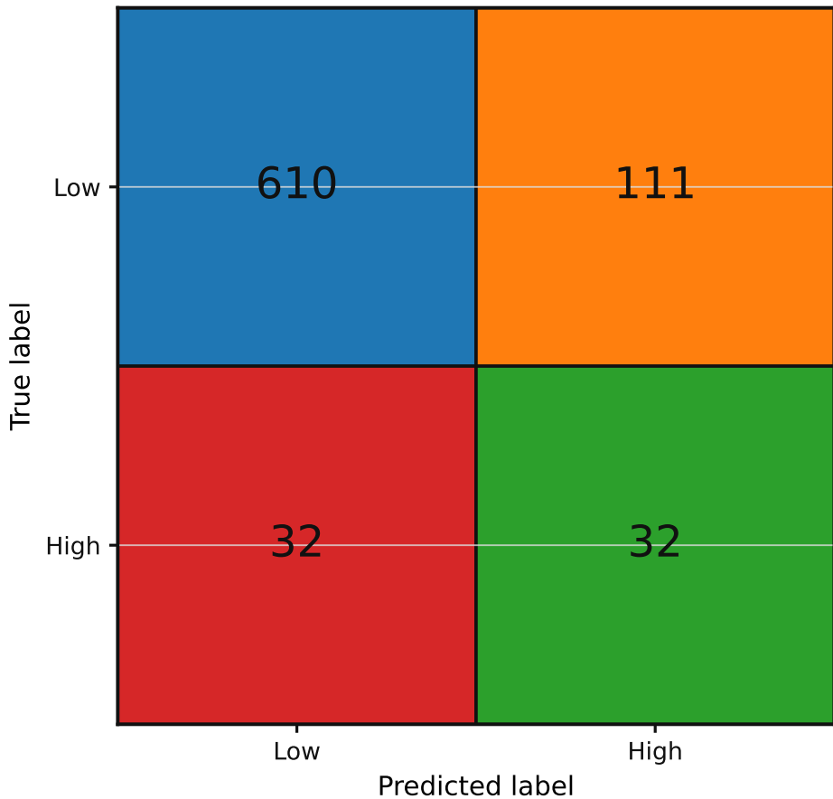
PPG-DaLiA Confusion Matrix - Predictive-only (B2)
