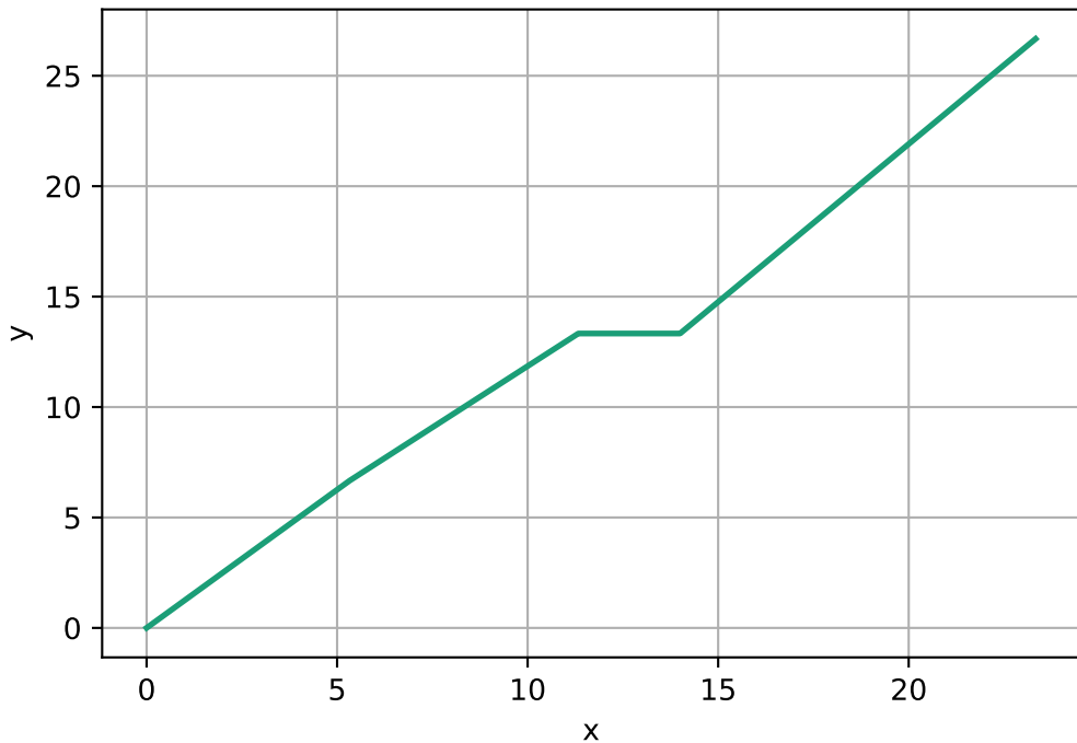
Multi-seed sanity
