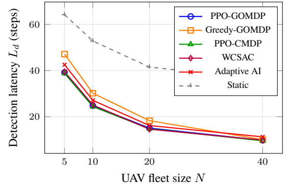
Figure 4: Detection latency L_d vs. UAV fleet size N ( n=20 seeds); error bars are \pm 1 SD. The Static curve is consistent with the Tarigan et al. (Tarigan, Robet, and Tarigan 2026) IoT figure ( \approx 45 steps; context only, non-comparable).
