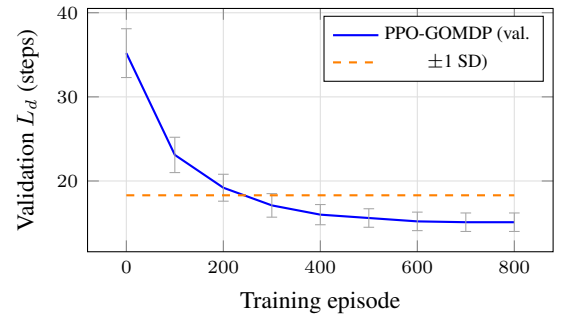
Figure 3: PPO-GOMDP learning curve: validation L_d (mean \pm 1 SD, 5 held-out seeds) vs. training episode; the governance invariant holds at 100% throughout (Corollary 1).
