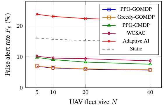
Figure 2: False public alert rate F_p vs. fleet size N under synthetic anomaly injection ( n=20 seeds). Holm–Bonferroni-corrected p < 0.01 for all GOMDP vs. non-GOMDP comparisons.
