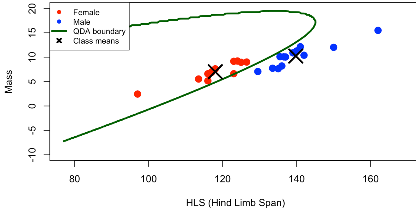
QDA: Curved Decision Boundary (HLS + Mass)
