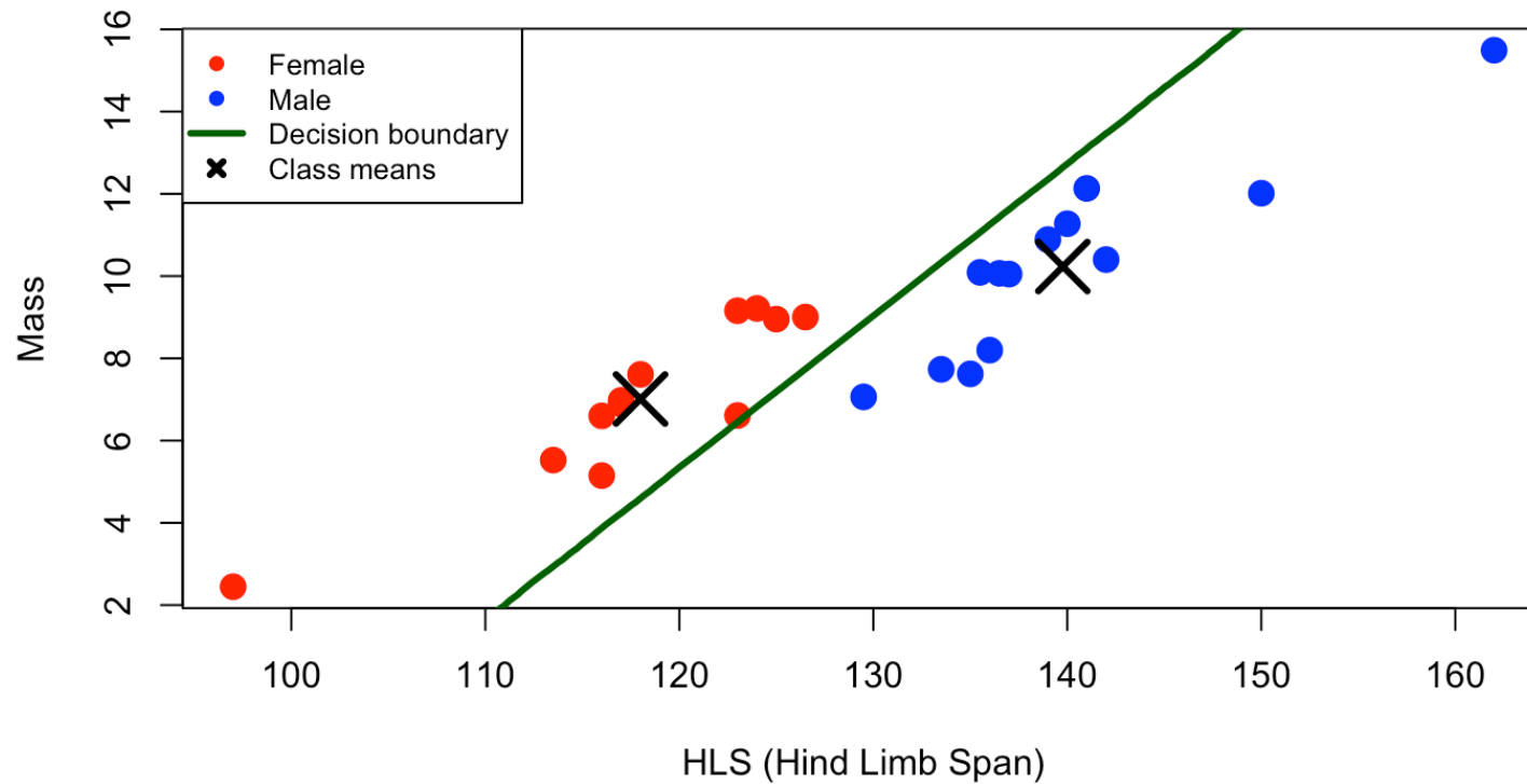
Bivariate LDA: Decision Boundary (Uniform Prior)
