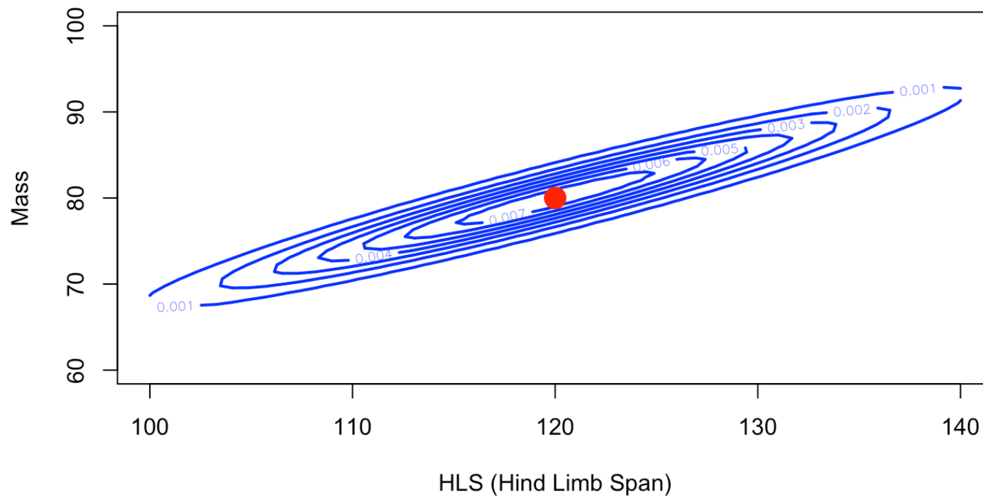
Bivariate normal with positive correlation
