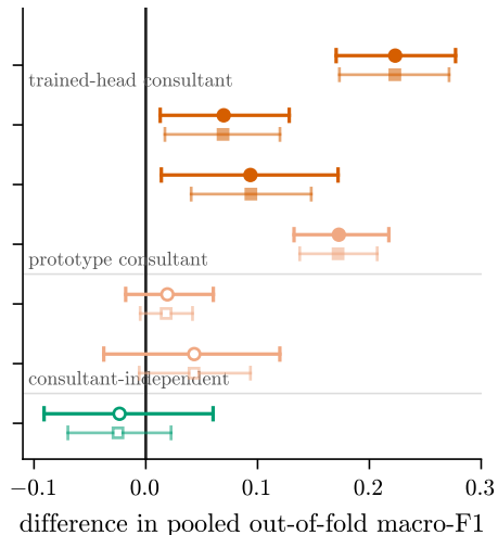
NF-ToN-IoT
