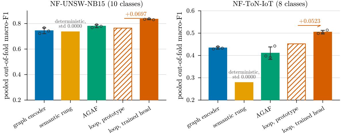
Error bars are training-seed variance at a fixed fold partition; fold-partition variance is not measured. Open circles are the three individual seeds. The consultant change is a point estimate; the two loop versions also differ in their selected top-k (31 to 29, and 25 to 16). The two panels have independent y-axes and are not comparable.
