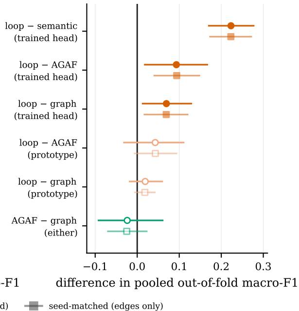
NF-ToN-IoT
