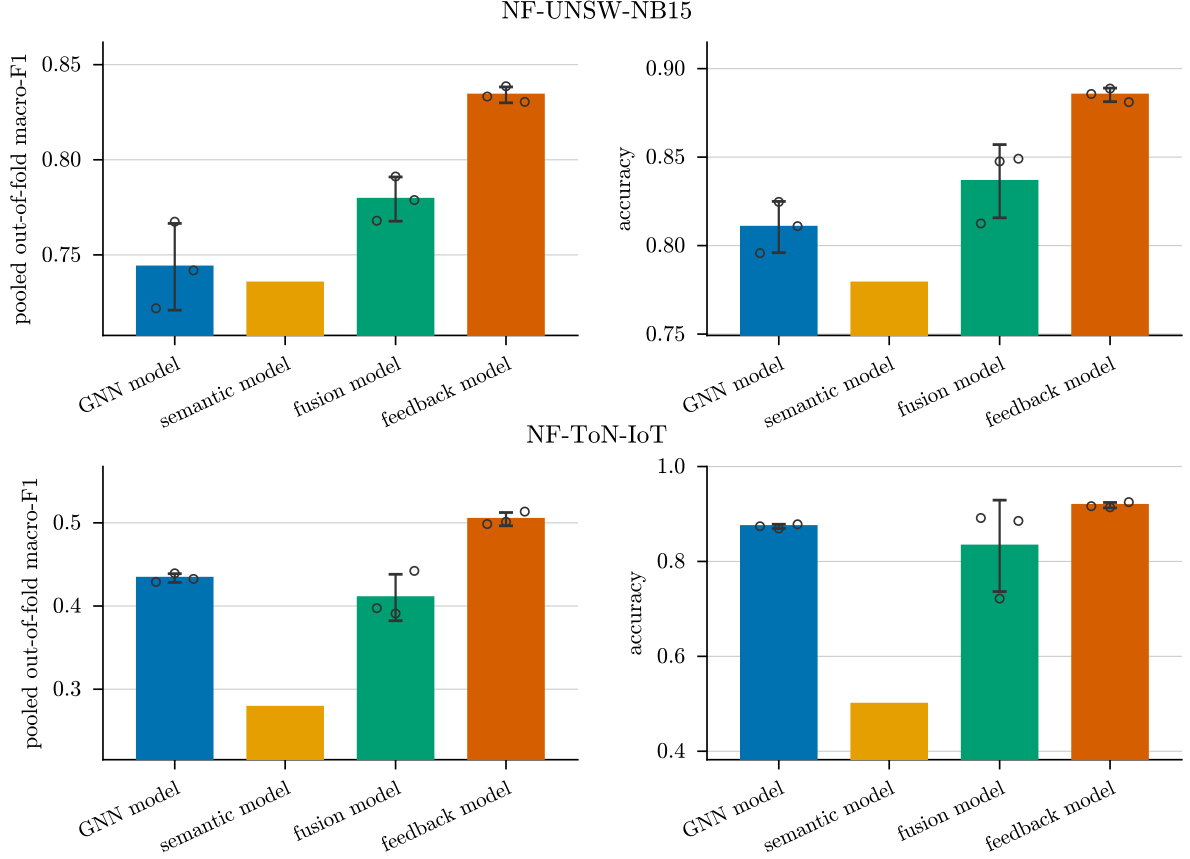
Left column macro-F1, right column accuracy, both on the rows the metric scores. Error bars are training-seed variance at a fixed fold partition; open circles are the three seeds. The semantic model is deterministic and has none. Every panel has its own y-axis. On NF-ToN-IoT the benign class holds 82% of scored edges, so accuracy stays high for every graph rung while macro-F1 separates them.
