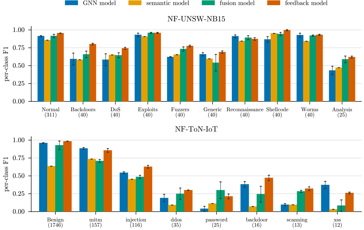
Three-seed means with training-seed standard deviations; classes are ordered by edge count, given under each label. The feedback model consults the trained head. No per-class difference carries an interval, and on the smallest classes a single edge moves F1 substantially.
