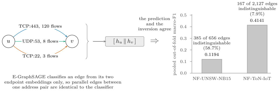
Not a training-schedule artifact: at the authors’ full 4,999 epochs on fold 0, validation macro-F1 plateaus near 0.11. Both bars are drawn in grey because neither is one of our rungs.
