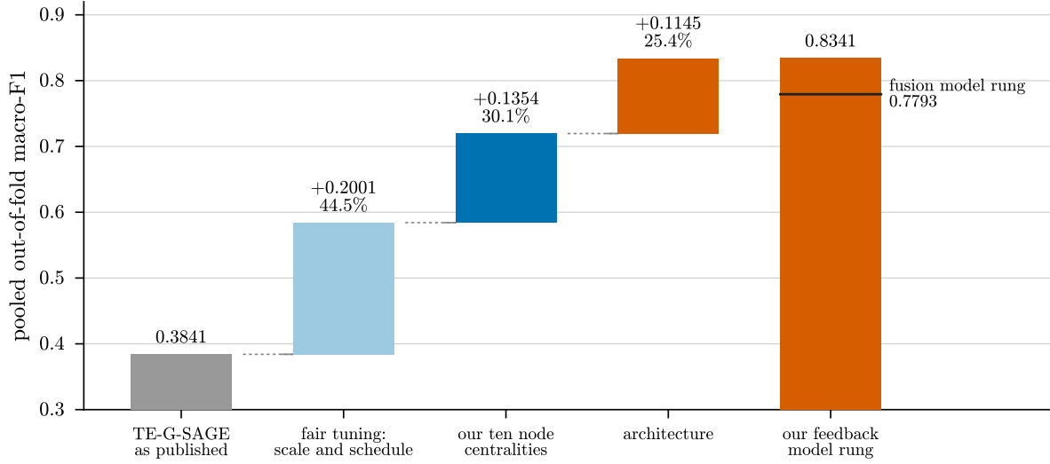
Point estimates only; every level is a three-seed mean and no step carries an interval or a separation claim.
