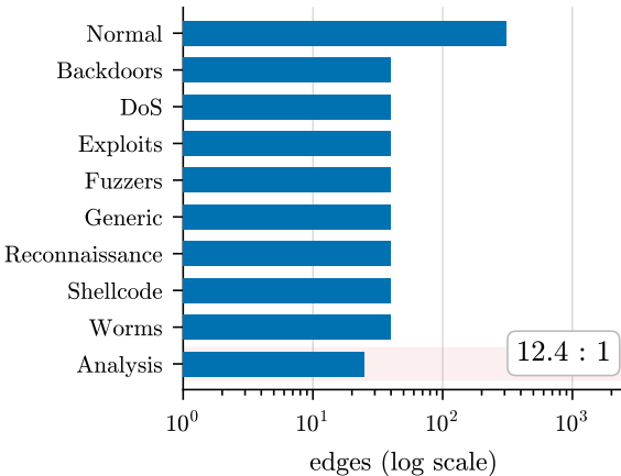
NF-UNSW-NB15, 656 edges
