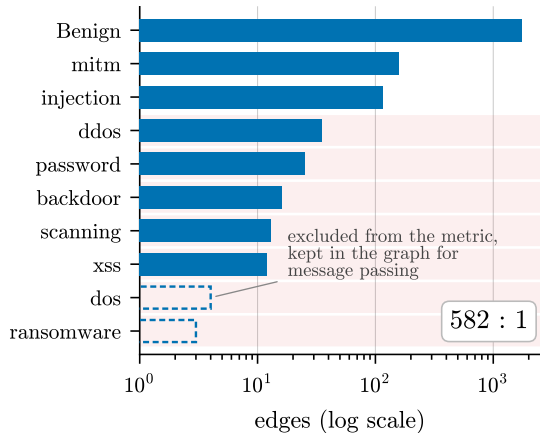
NF-ToN-IoT, 2,127 edges
