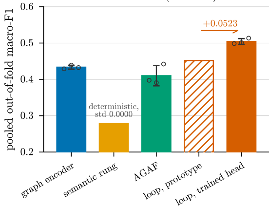
NF-ToN-IoT (8 classes)
