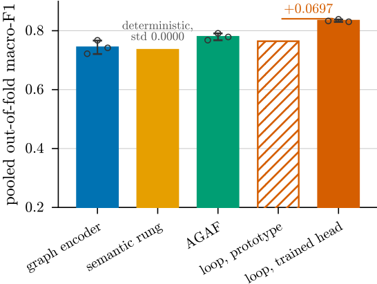
NF-UNSW-NB15 (10 classes)
