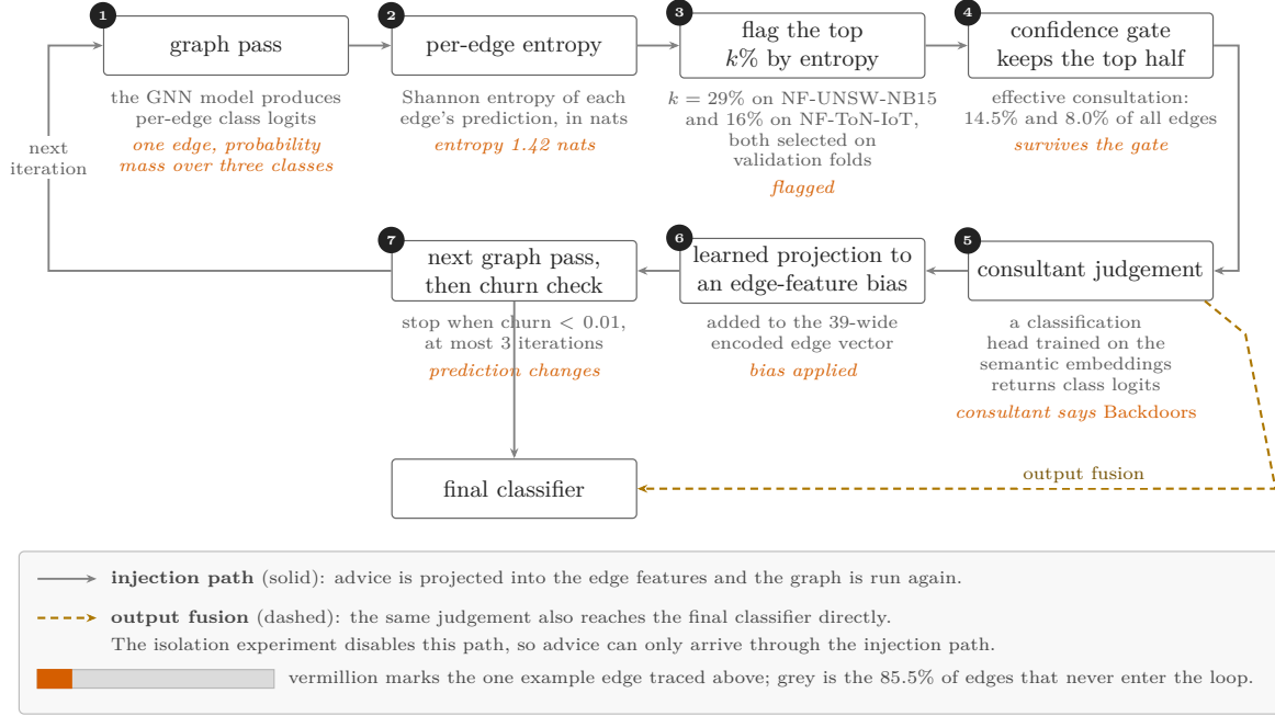
Figure 3: One pass of the feedback model. The solid path is the injection mechanism under test: the consultant’s judgement is projected into the 39-wide encoded edge vector and the graph is run again. The dashed path is output fusion, which reaches the final classifier without passing through the graph, and which the isolation experiment of Section 4.3 disables. The percentages are the selected entropy thresholds and the effective consultation rates they produce.
