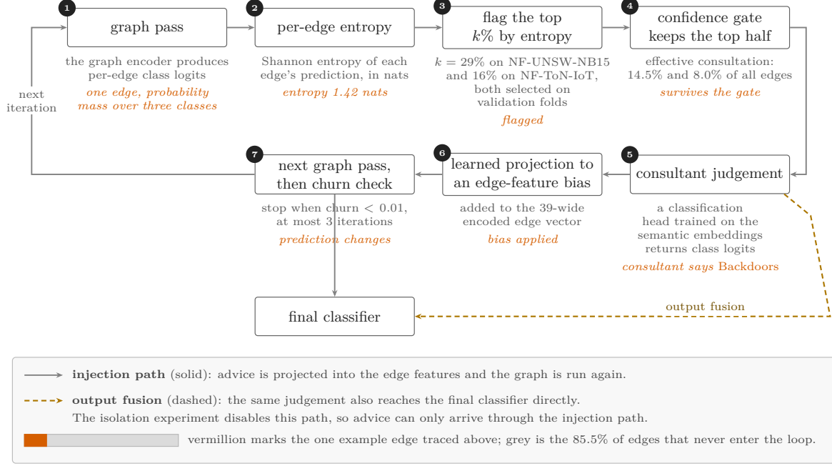
Figure 3: One pass of the feedback feedback model. The solid path is the injection mechanism under test: the consultant’s judgement is projected into the 39-wide encoded edge vector and the graph is run again. The dashed path is output fusion, which reaches the final classifier without passing through the graph, and which the isolation experiment of Section 4.3 disables. The percentages are the selected entropy thresholds and the effective consultation rates they produce.
