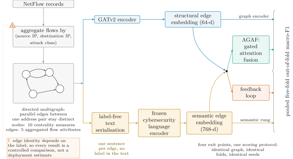
Figure 1: The pipeline, from flow records to four scored rungs. Blue is the structural branch, orange the semantic branch, green the fusion stage and vermillion the feedback feedback model. Every rung is an exit point from one shared graph and is scored by one protocol on one fold partition and one set of seeds. The marked aggregation step is the label-conditioned grouping key that bounds every claim in this report.
