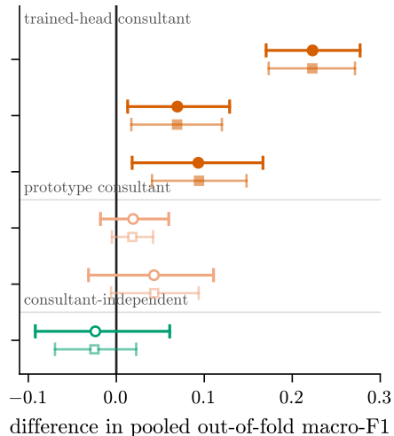
NF-ToN-IoT
