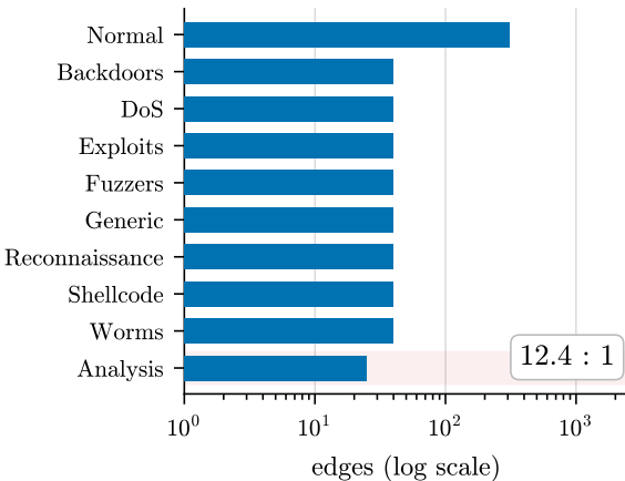
NF-UNSW-NB15, 656 edges
