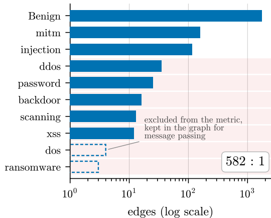
NF-ToN-IoT, 2,127 edges
