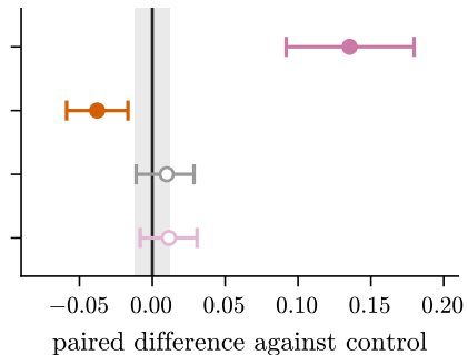
NF-ToN-IoT
