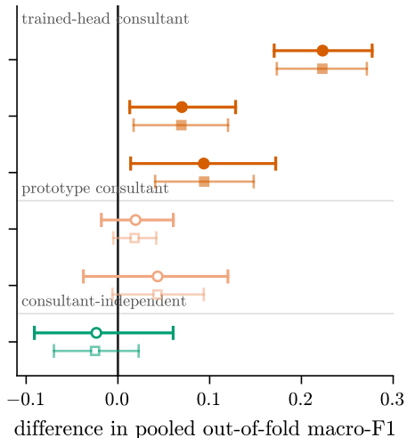
NF-ToN-IoT
