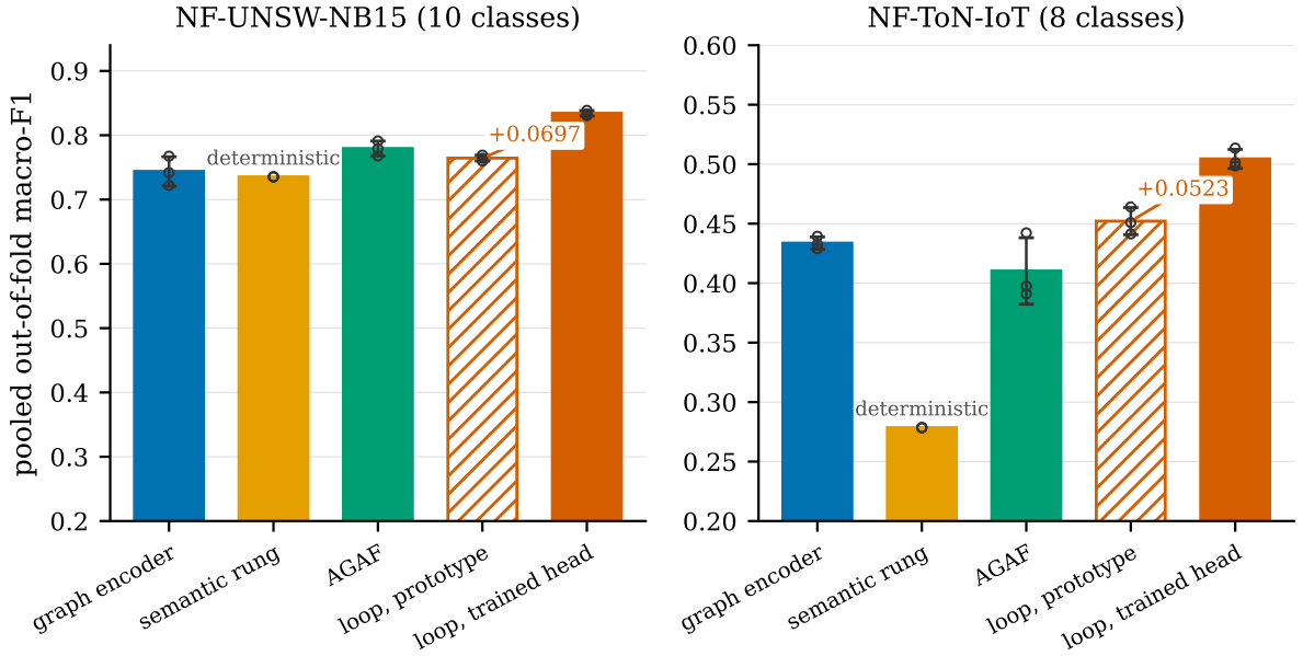
Error bars are training-seed variance at a fixed fold partition; open circles are the three seeds. The two panels have independent axes: the datasets score different numbers of classes and their levels are not comparable.
