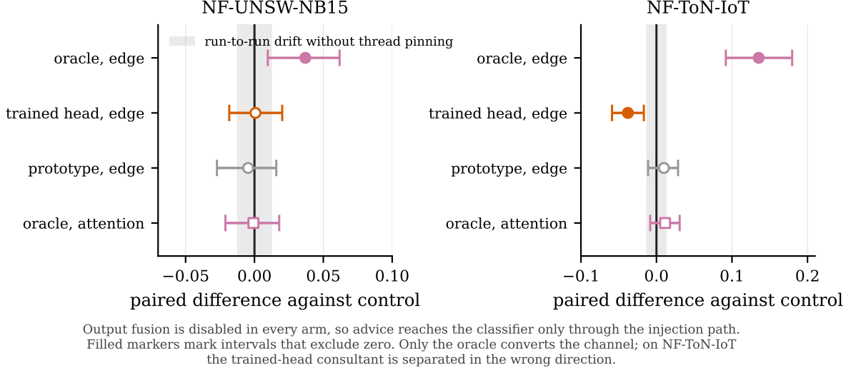
Figure 4: The mechanism in isolation, output fusion disabled in every arm. Only the oracle converts the channel. The shaded band is the run-to-run drift measured without thread pinning.
