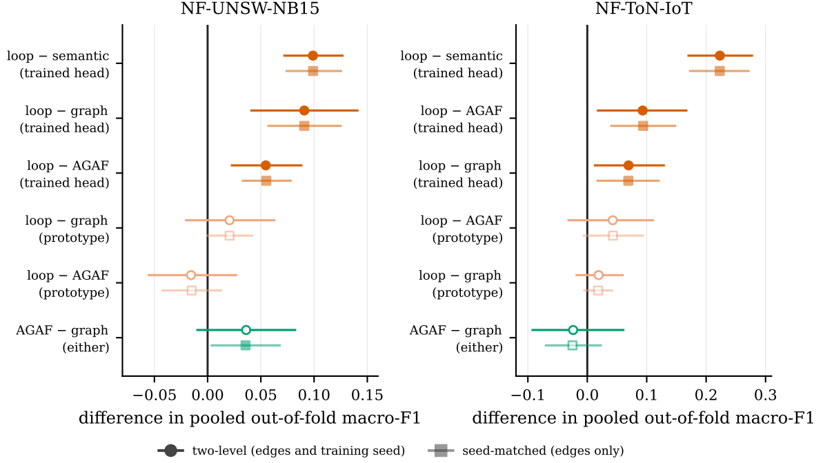
Filled markers mark intervals that exclude zero. Every loop comparison clears zero under the trained-head consultant and none does under the prototype. The two-level interval is the one the decision rule uses.
