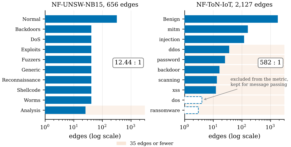
Figure 1: Class sizes on a logarithmic axis. The two graphs differ by roughly a factor of 47 in most-to-least-frequent class ratio, which is the axis the cross-dataset comparison turns on.
