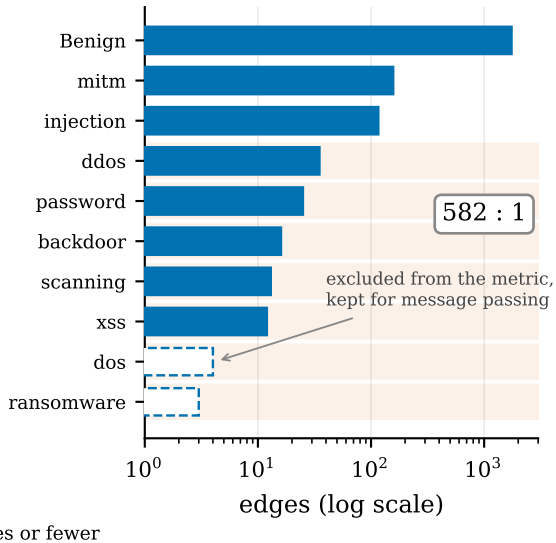
NF-ToN-IoT, 2,127 edges
