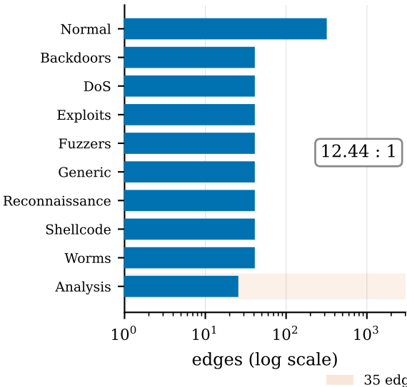
NF-UNSW-NB15, 656 edges
