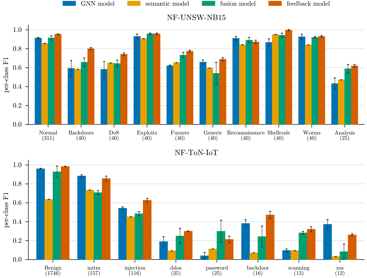
Three-seed means with training-seed standard deviations; classes are ordered by edge count, given under each label. The feedback model consults the trained head. No per-class difference carries an interval, and on the smallest classes a single edge moves F1 substantially.
