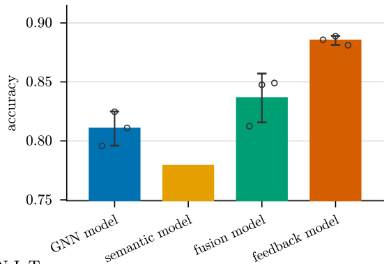
NF-ToN-IoT
