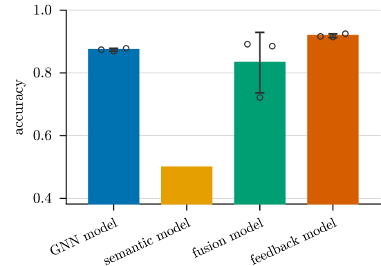
NF-ToN-IoT
