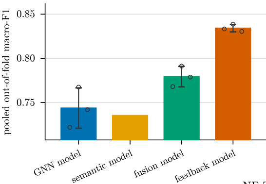
NF-ToN-IoT
