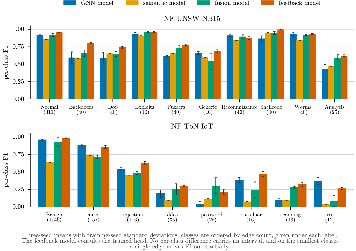
Figure 10: Per-class F1 for the four rungs, both datasets, with classes ordered by edge count and the count under each label. The feedback model is the canonical one, consulting the trained head. Error bars are one standard deviation over three training seeds at a fixed fold partition. No per-class value carries an interval, and on the smallest classes a single edge moves F1 substantially.
