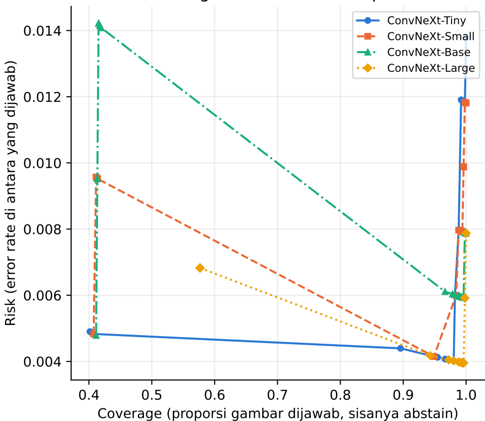
Risk-Coverage Curve -- selective prediction
