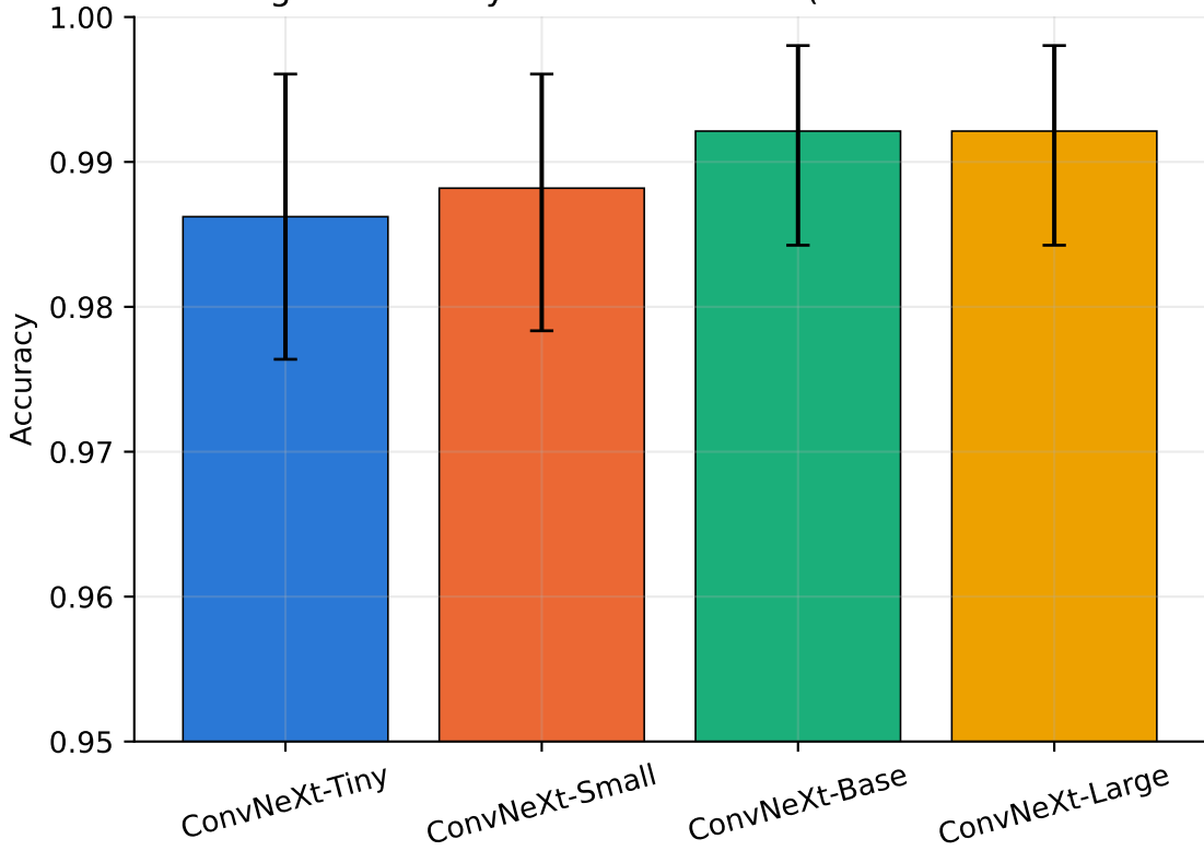
Perbandingan Accuracy antar Backbone (bar = 95% CI bootstrap)
