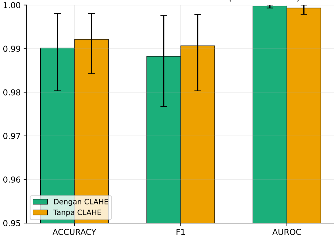
Ablation CLAHE -- ConvNeXt-Base (bar = 95% CI)
