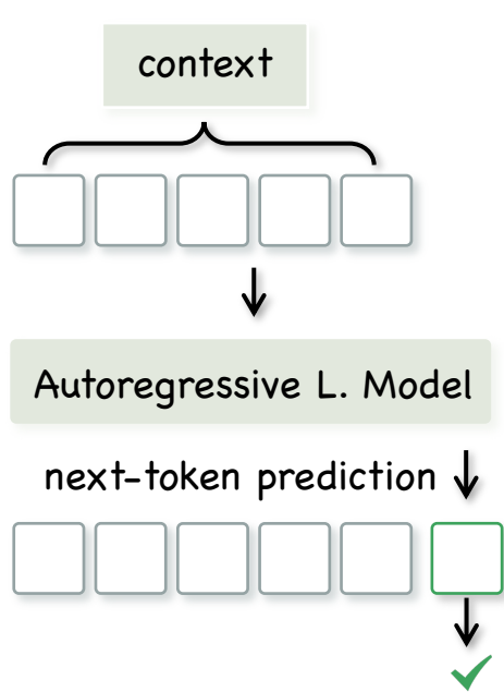
(b) AR
