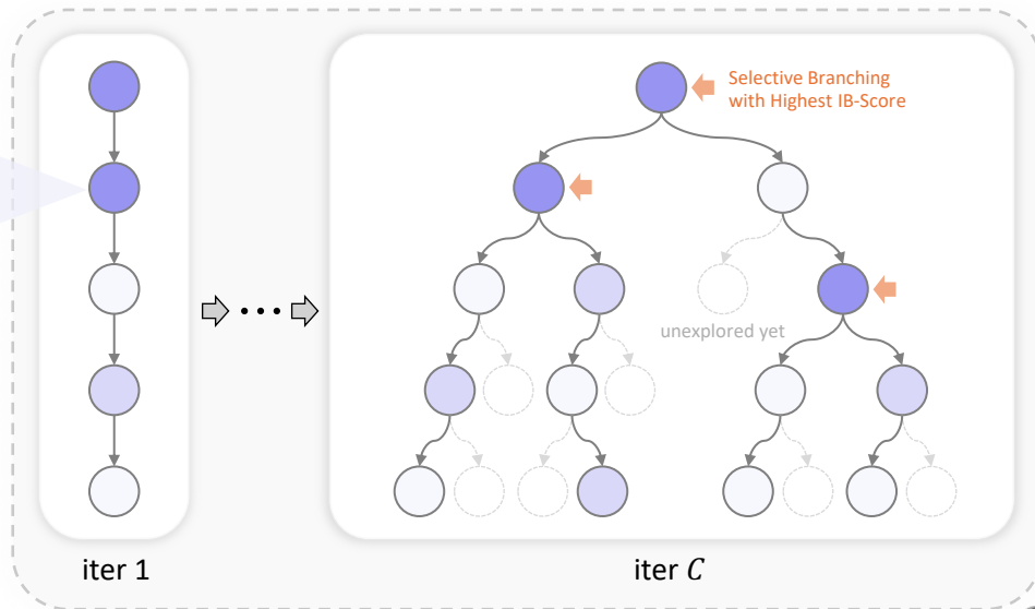
Information Bottleneck Guided Tree Search (IBTree)
