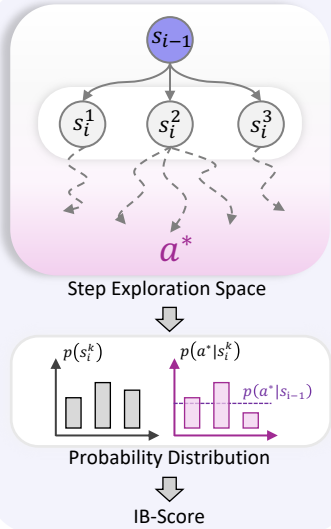
IB-Score Calculation
