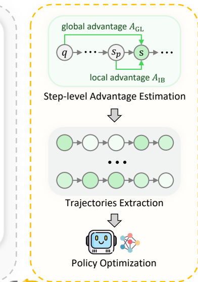
RL Training
