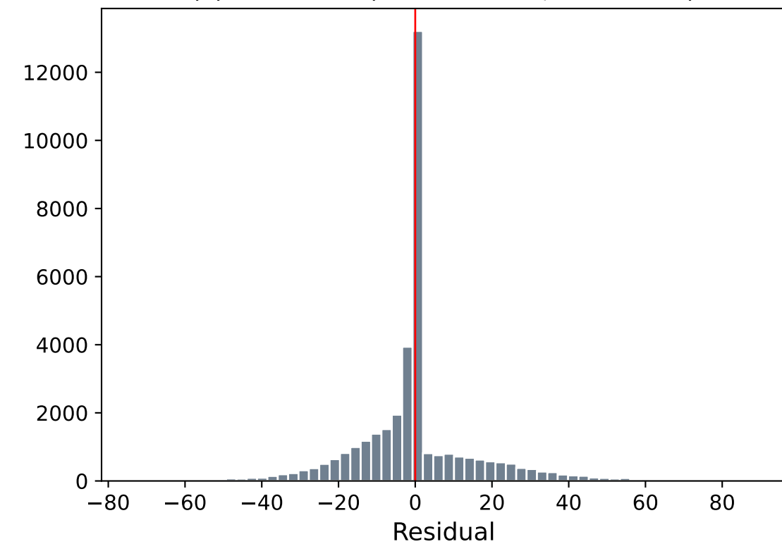
(c) Residuals (mean=-0.11, sd=16.03)
