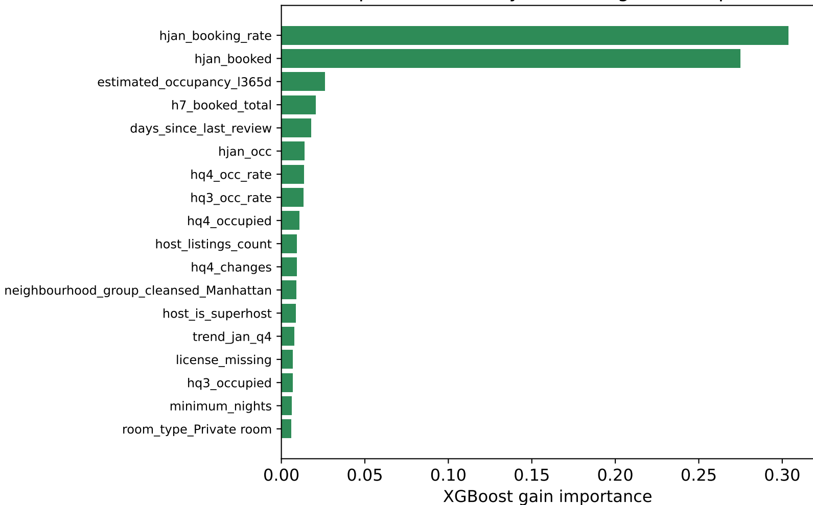
Top-18 features by XGBoost gain (Setup C)
