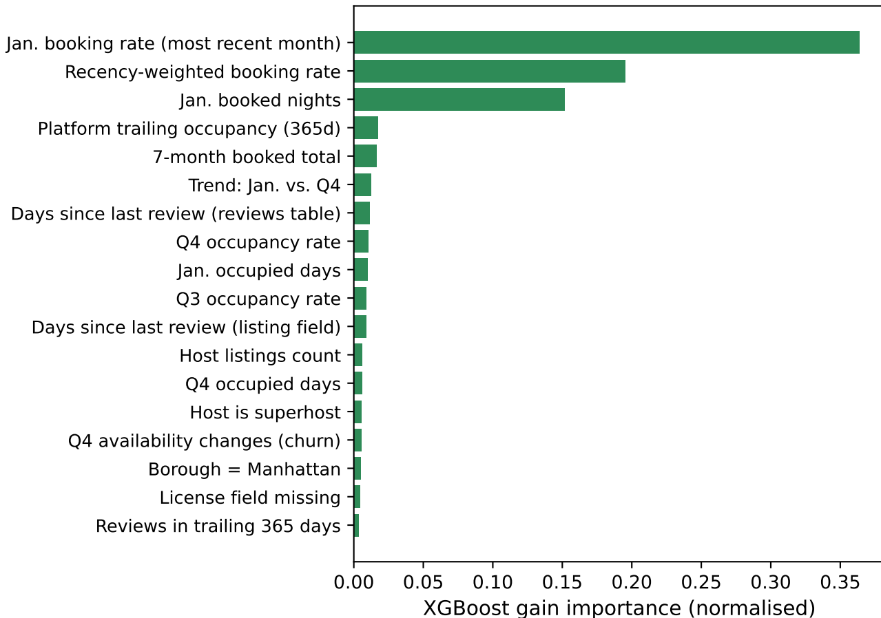
Top-18 features by XGBoost gain (Setup C)
