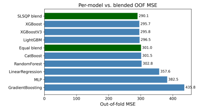
Out-of-fold MSE for each model and for the equal-weight vs. optimal (SLSQP) blends. The weighted blend is the best configuration.
