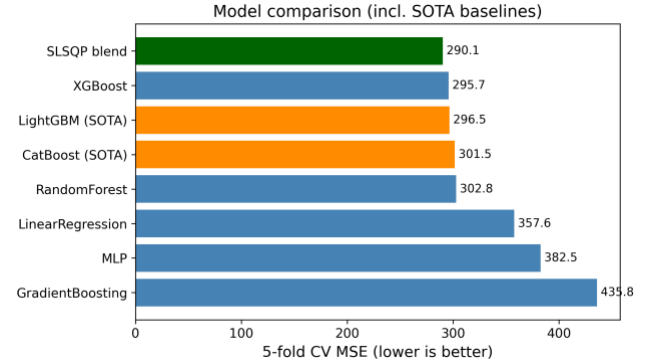
Model comparison by cross-validated MSE, including the LightGBM/CatBoost baselines and the final blend. The tree-based models cluster tightly at the top; Linear Regression, the MLP, and the untuned Gradient Boosting trail well behind.
