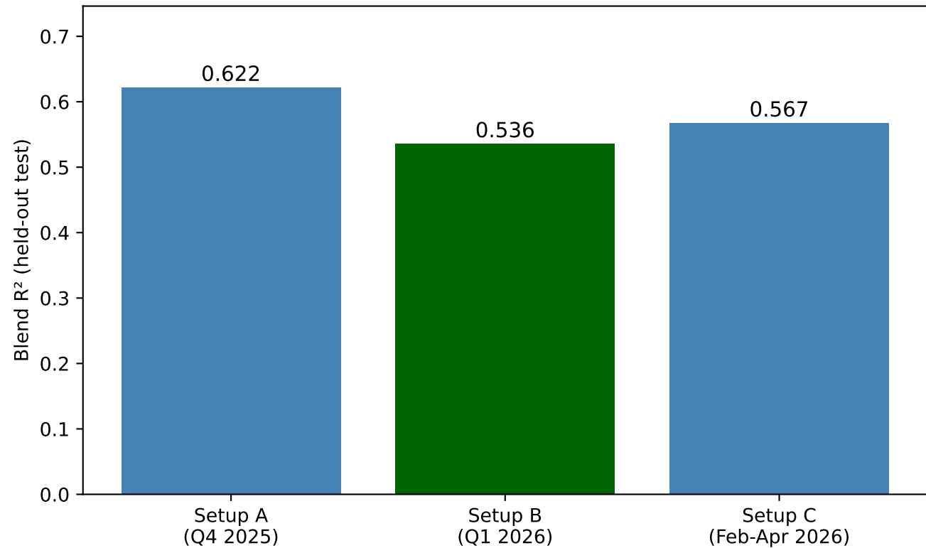
Cross-period robustness: blend held-out test R^2 by setup
