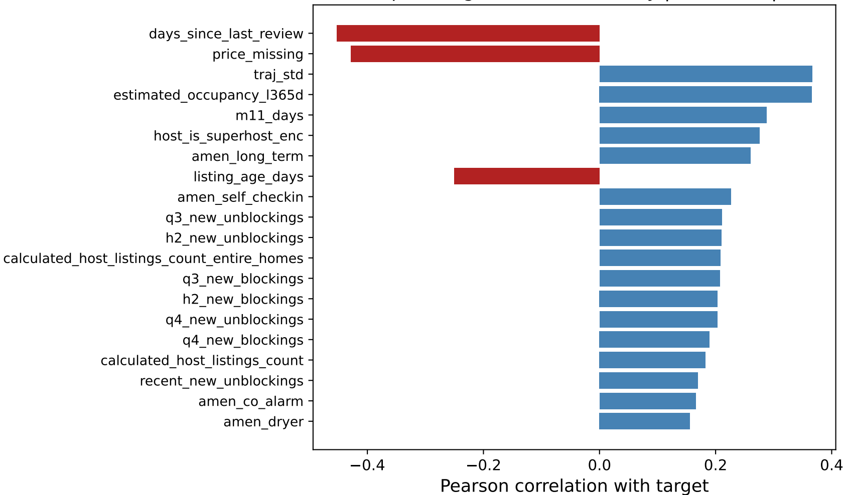
Top-20 engineered features by |correlation|
