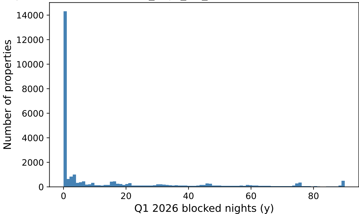
Target distribution: blocked_days_Q1_2026 (zero-inflated, bounded [0,90])
