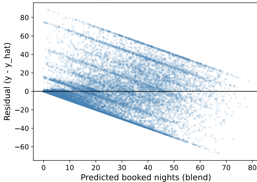
(c) Residual distribution (mean=0.13, sd=17.26)
