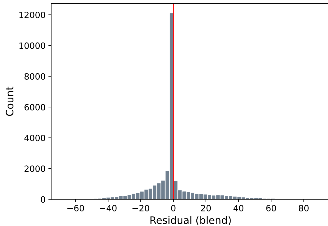
(c) Residual distribution (mean=0.13, sd=17.26)
