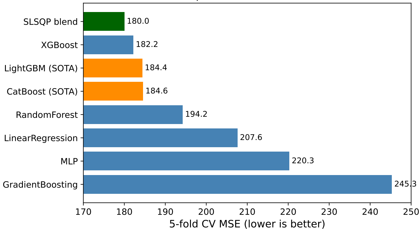
Model comparison (incl. SOTA baselines)
