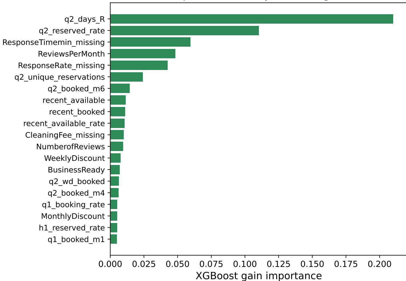
Top-20 features by XGBoost gain
