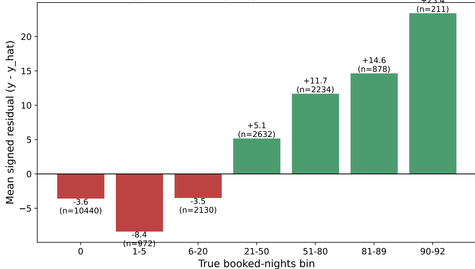
Systematic bias by target bin (blend, dev OOF)
