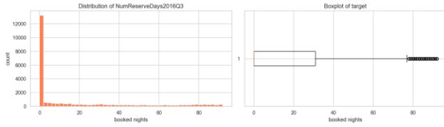
Distribution of the target (Q3 2016 booked nights). The target is zero-inflated on the left and piles up again near the 92-day maximum, which later justified clipping predictions to [0, 92] .
