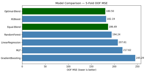
Out-of-fold MSE for each model and for the equal-weight vs. optimal (SLSQP) blends. The weighted blend is the best configuration.
