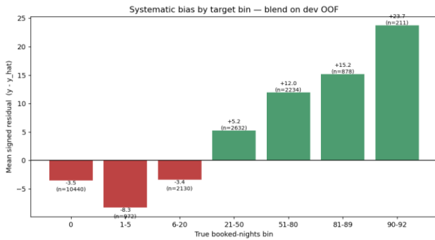
Mean signed residual ( y - \hat{y} ) by true booked-nights bin. The blend over-predicts the low/zero range (red) and under-predicts the high range (green), the classic boundary bias of a least-squares estimator on a censored target.
