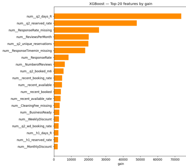
XGBoost gain-based feature importances. Behavioural and recency features dominate, in agreement with Fig. 2.
