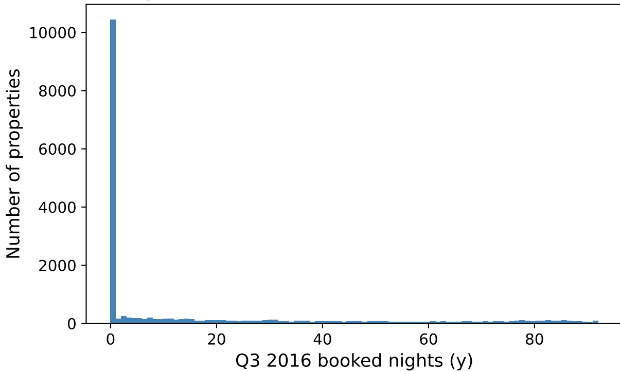
Target distribution (zero-inflated, bounded [0,92])
