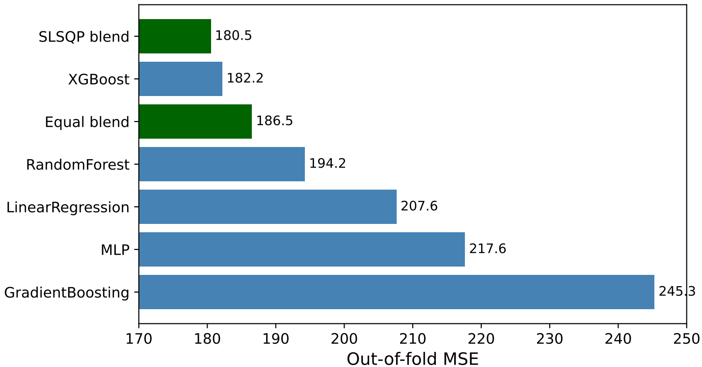
Per-model vs. blended OOF MSE
