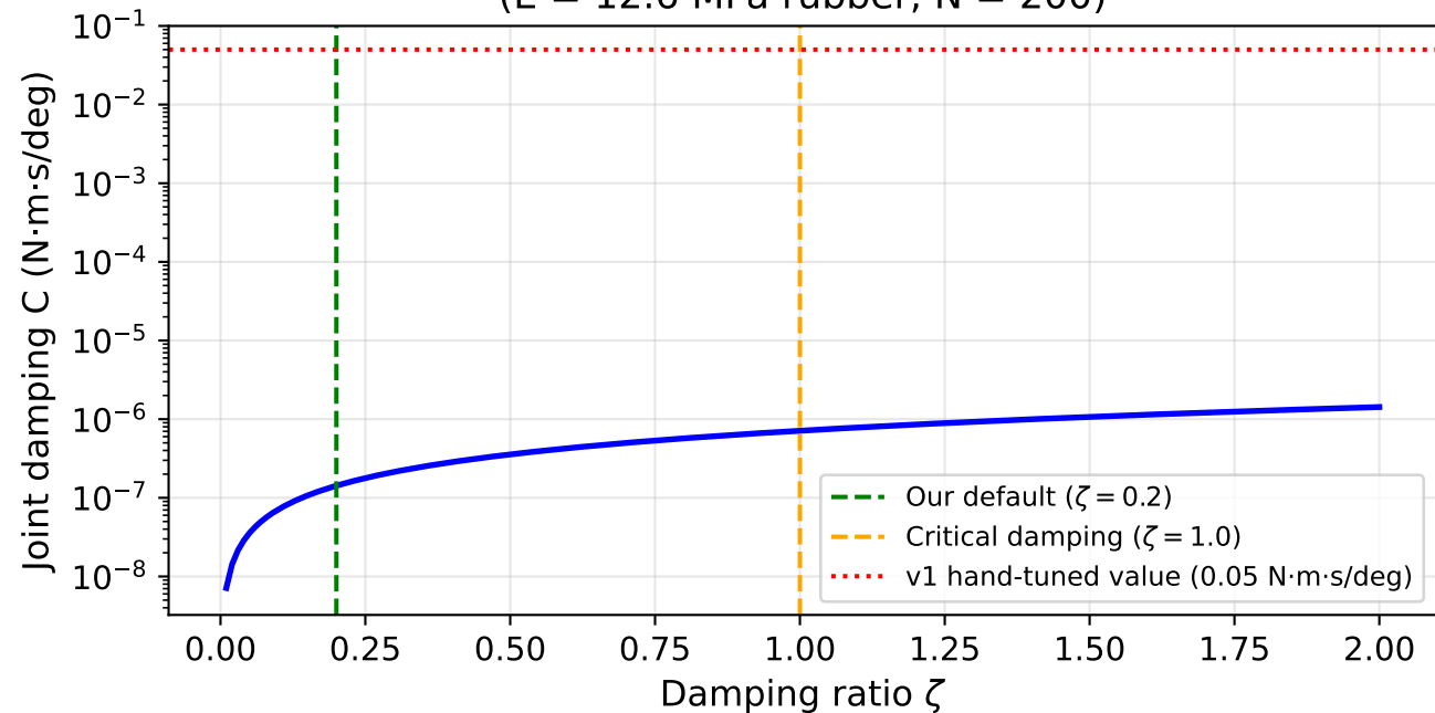
Joint damping vs. damping ratio ( E = 12.6 MPa rubber, N = 200 )
