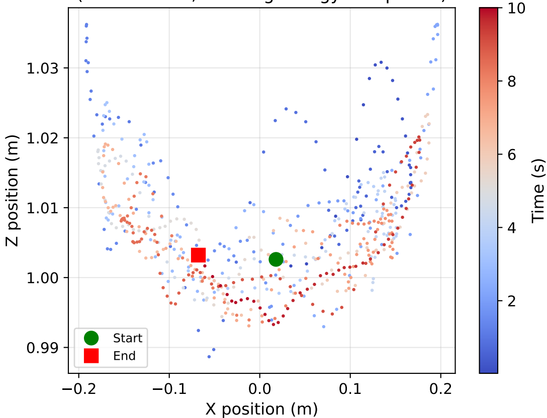
Cable tip trajectory in X-Z plane (color = time, showing energy dissipation)
