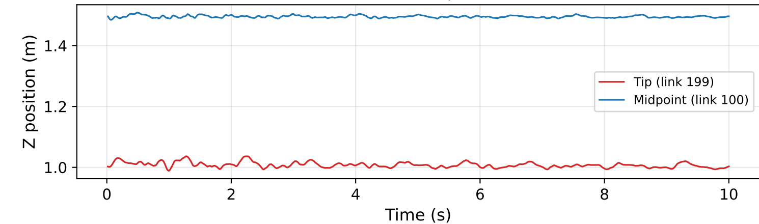
Cable vertical position
