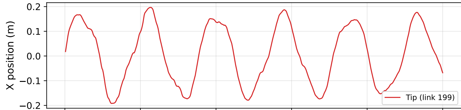
Cable tip lateral displacement
