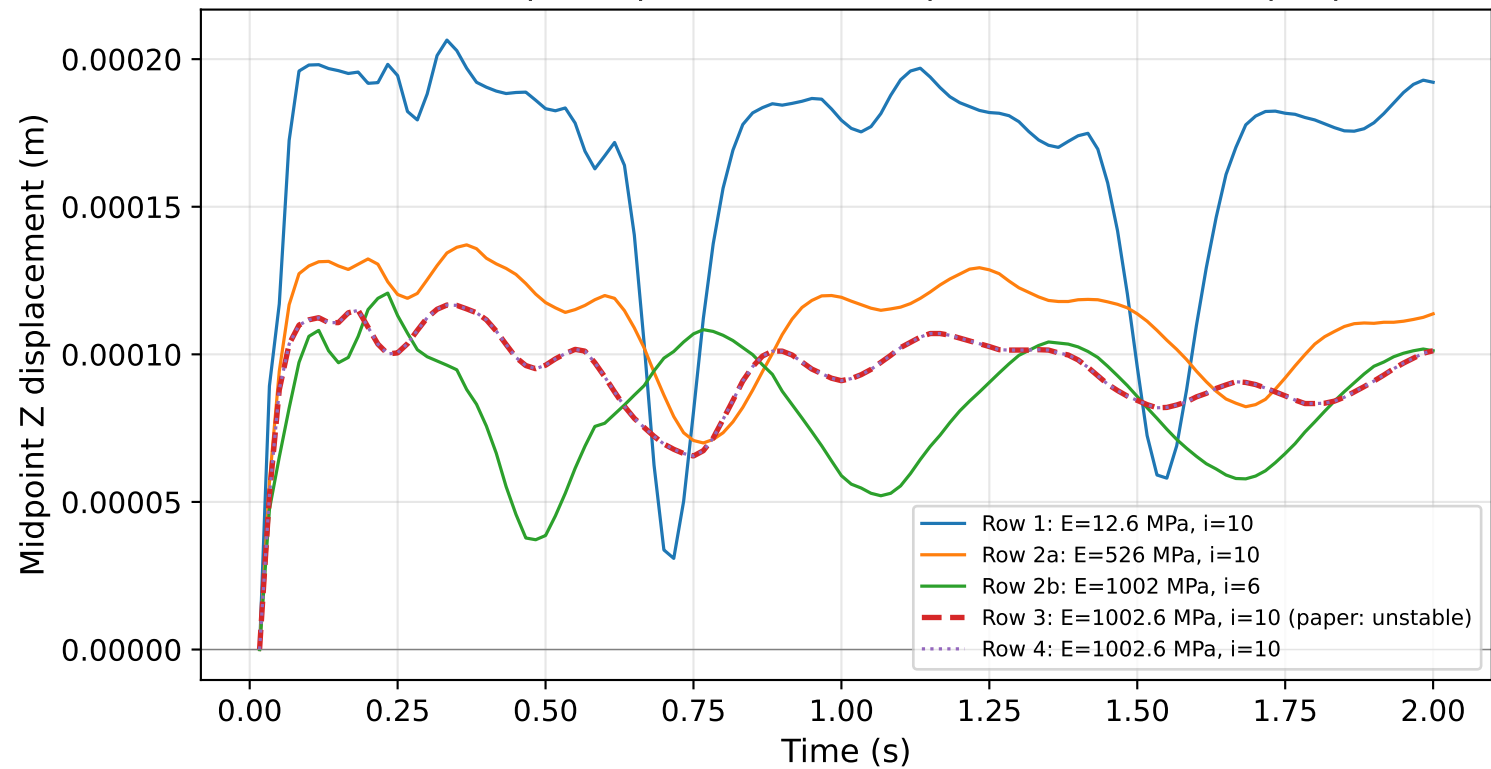
Govoni sweep: midpoint vertical displacement after step input
