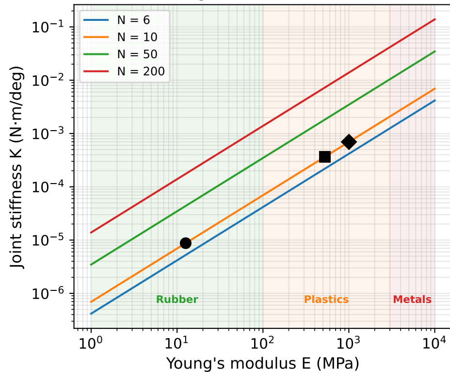
Bending stiffness vs. material
