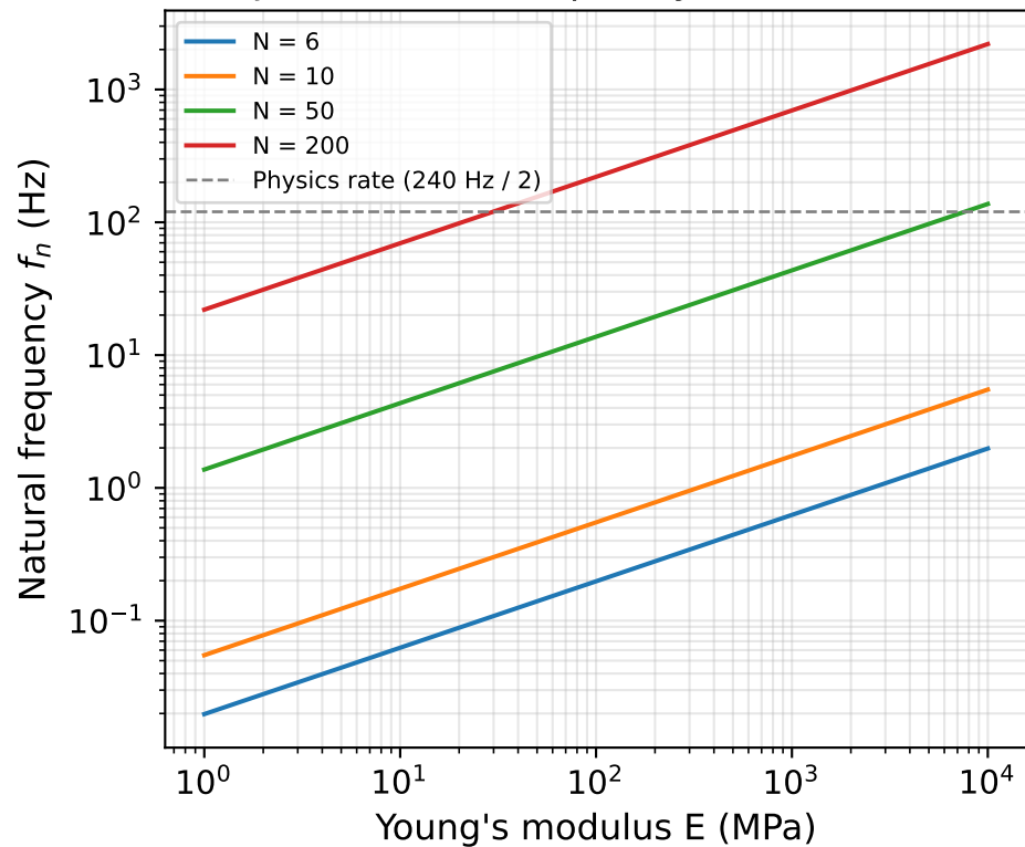
Joint natural frequency vs. material
